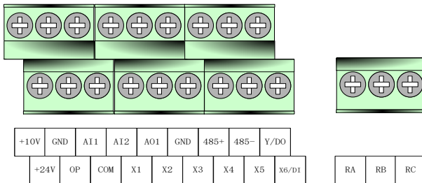
Figure 3-5 DV203 series inverter control circuit terminal layout
