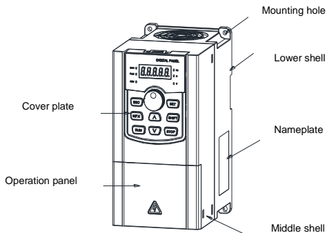
Figure 2-3 DV203 series plastic case appearance diagram
