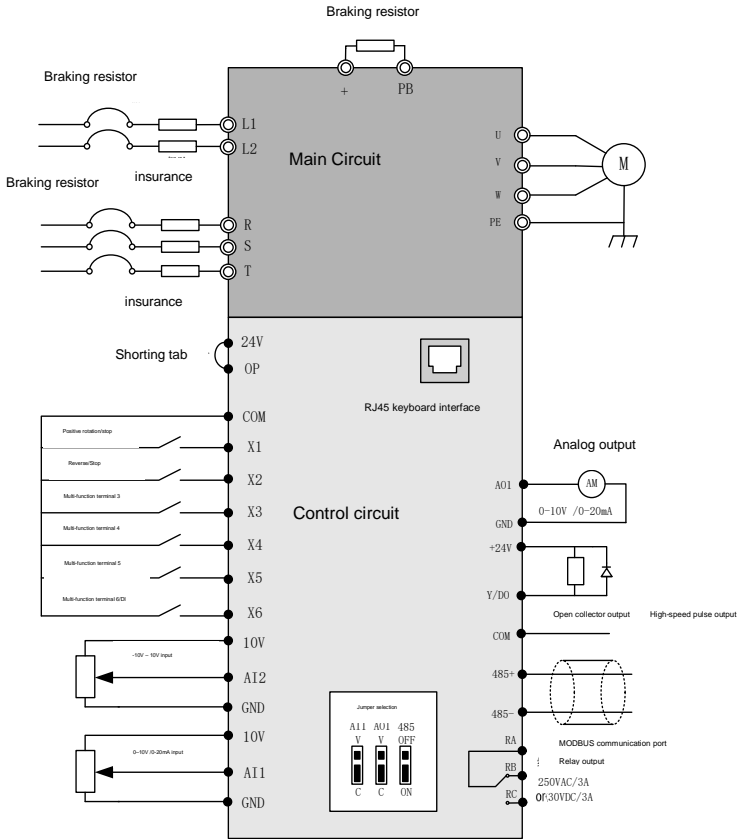
Figure 3-2 Typical wiring diagram of DV203 products
