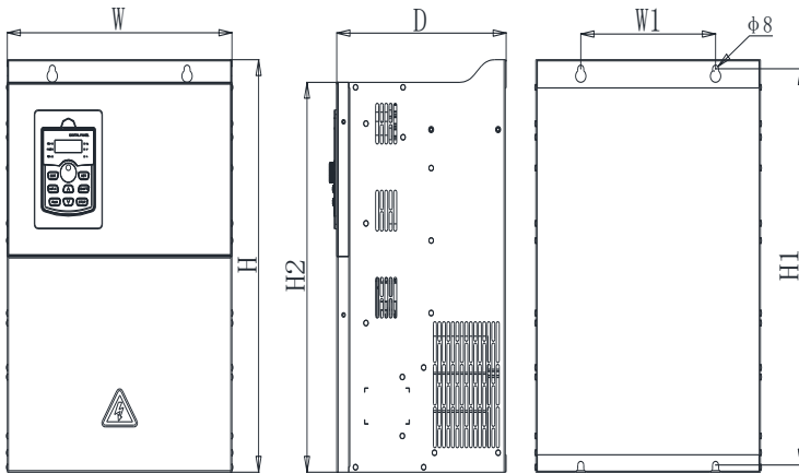
Figure 2-5 DV203 Series Sheet Metal Housing Mounting Hole Dimension Diagram
