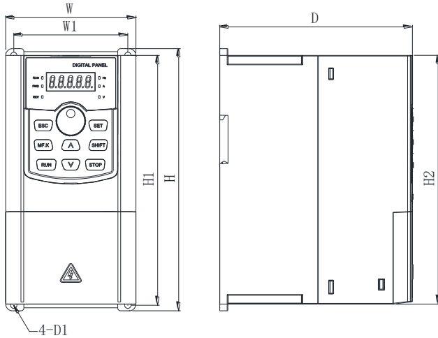
Figure 2-4 Plastic shell mounting hole size diagram
