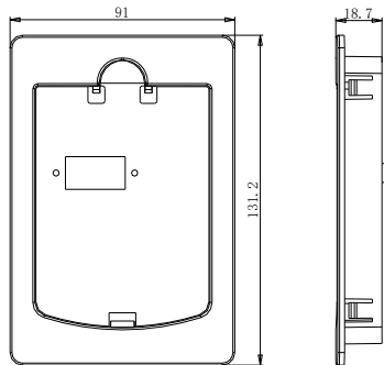
Figure 2-5 External keyboard 1 mounting base external dimensions
