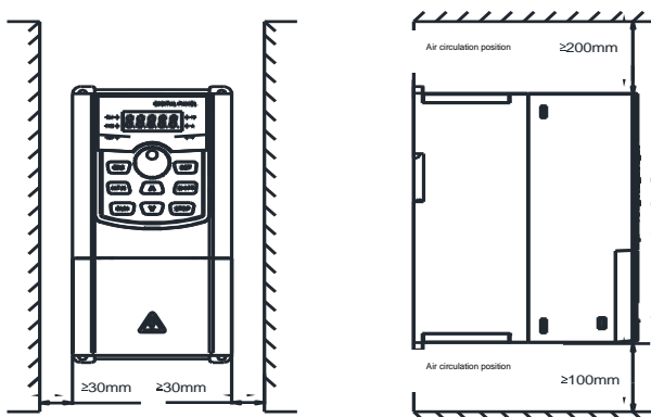
Figure 3-1 Installation diagram of DV203 series inverter
