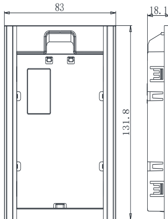
Figure 2-7 External keyboard 2 external dimensions
